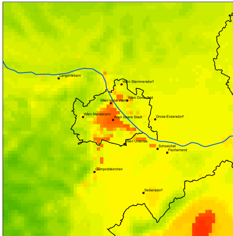
Tropical Nights ( T_{min} > 20^{\circ} C ) Mean 2031-2060
