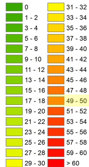
Tropical Nights ( T_{min} > 20^{\circ} C ) Mean 2031-2060
