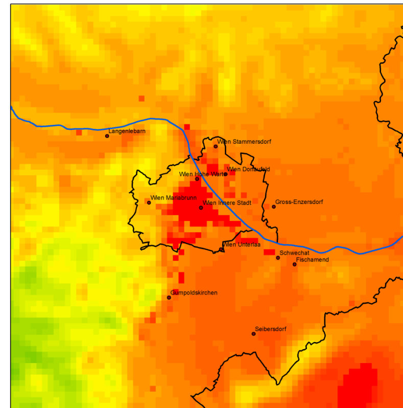
Tropical Nights ( T_{min} > 20^{\circ} C ) Mean 2071-2100
